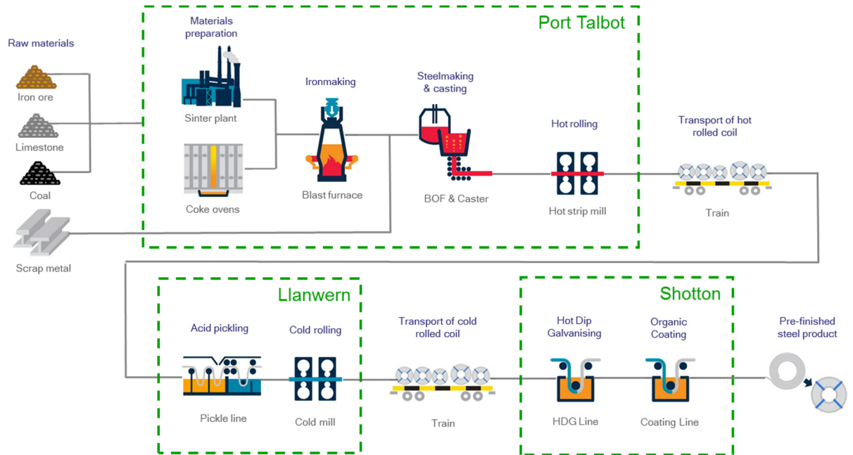
Figure 1 Process overview from raw materials to pre-finished steel
