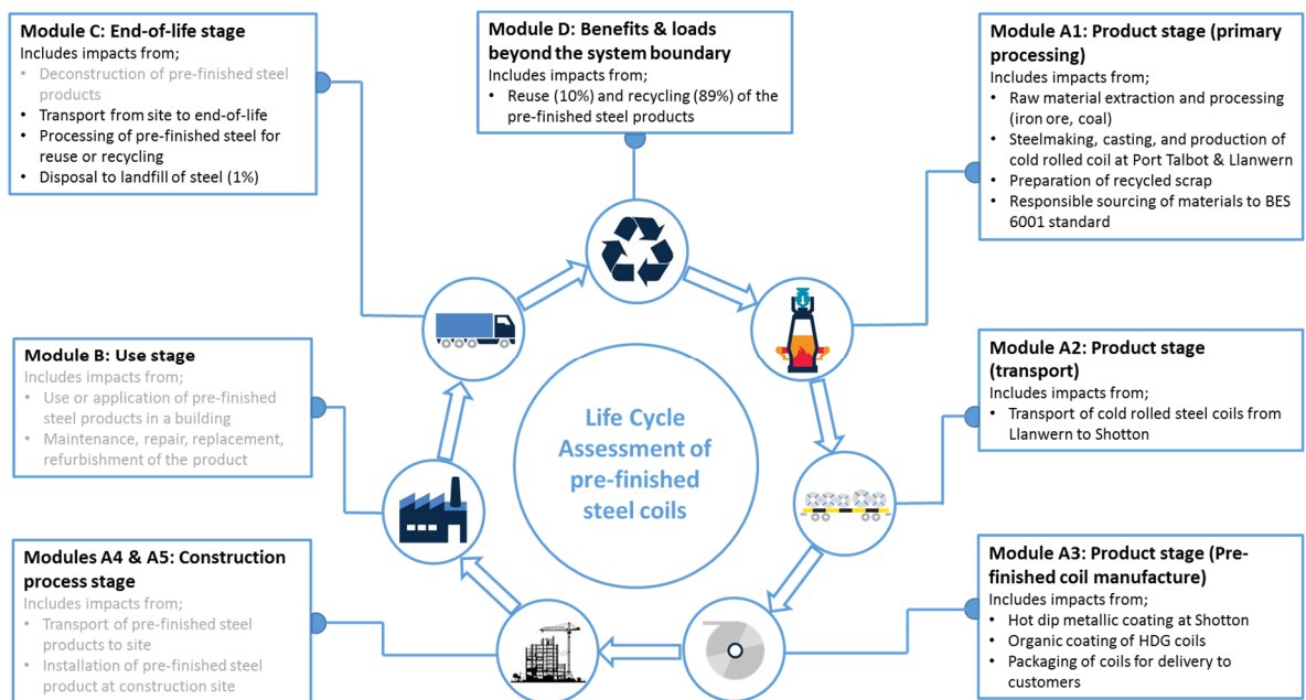
Figure 2 Life cycle assessment of pre-finished steel
