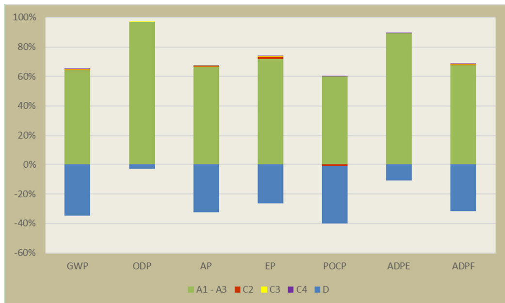
Figure 3 LCA results for the pre-finished steel
